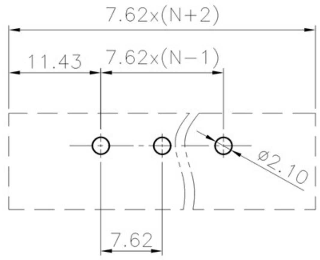
PCB LAYOUT
